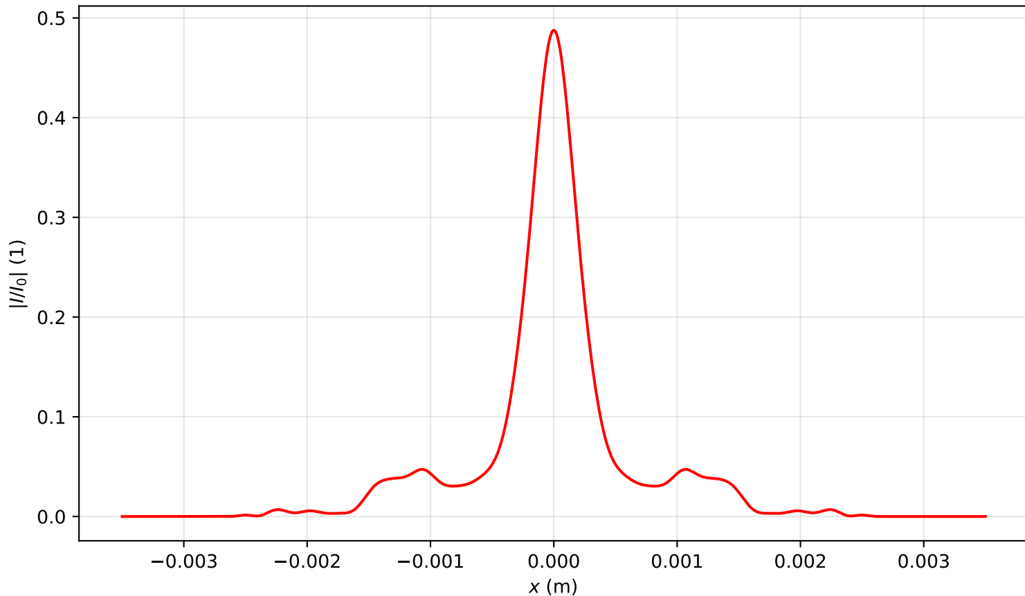
Intensity profile I(x, y = 0, z = 3.105)/I_0 , P_{in}=5.0P_{cr} , artificial time
